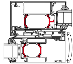
BSC94 Mono Rail Standard Interlock
